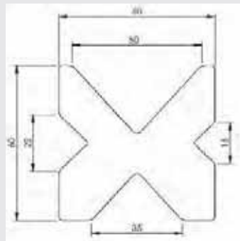
PIC: 4V LOWER DIE
