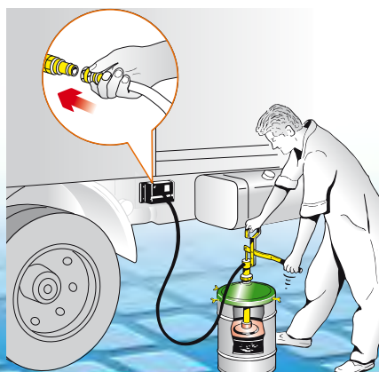
Filling central greasing system
